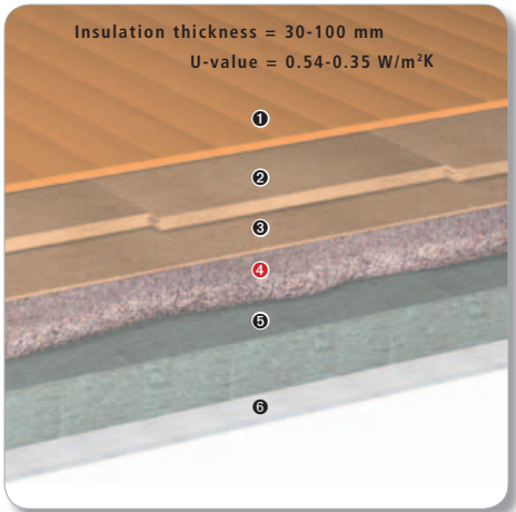
Storey Ceiling DB14 Solid ceiling
