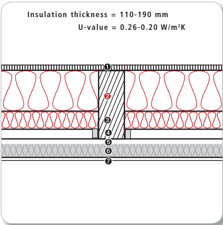
Storey Ceiling DB13 Wooden beam ceiling, old stock
