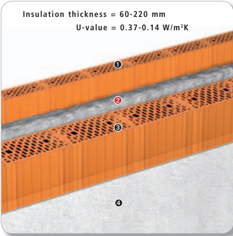
Outside Wall with Core Insulation W13
